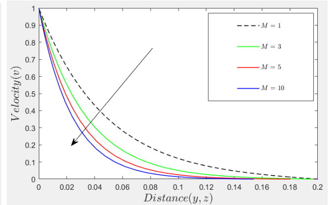
Figure 5.16: Velocity profiles ( v ) for different values of M .
