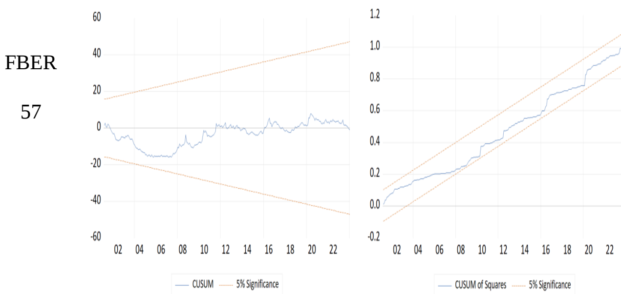
Fig. 3. CUSUM and CUSUM of Squares Test
